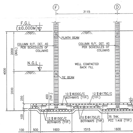
SECTION 1-1 (SCALE 1:50)
