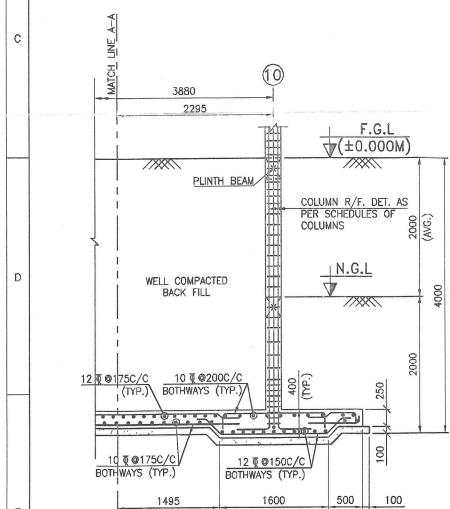
SECTION 1-1 (SCALE 1:50)
