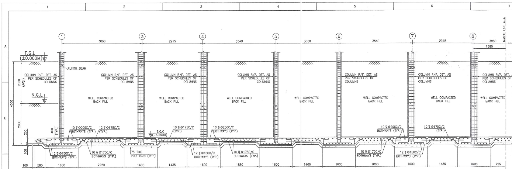
SECTION 1-1 (SCALE 1:50)
