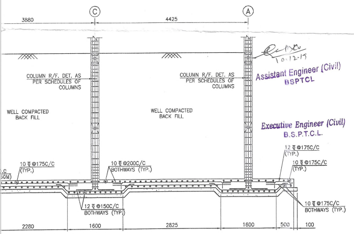
SECTION 2-2 (SCALE 1:50)
